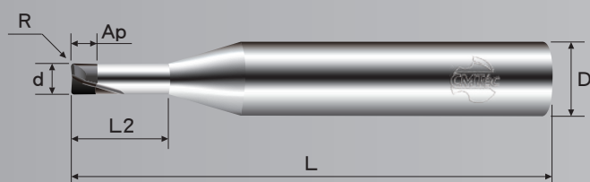
PCBN圓鼻銑刀 | PCBN Corner Radius End Mills
