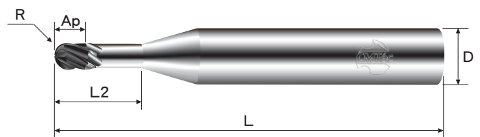
PCD球刀 | PCD Ball Nose End Mills
