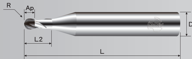
PCBN球刀 | PCBN Ball Nose End Mills
