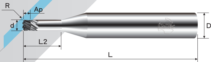
PCD圓鼻銑刀 | PCD Corner Radius End Mills
